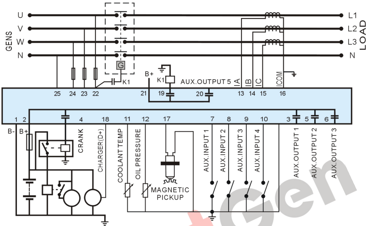
HGM420N Typical wiring diagram
